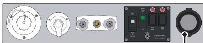
Shore Power Cord Hookup
